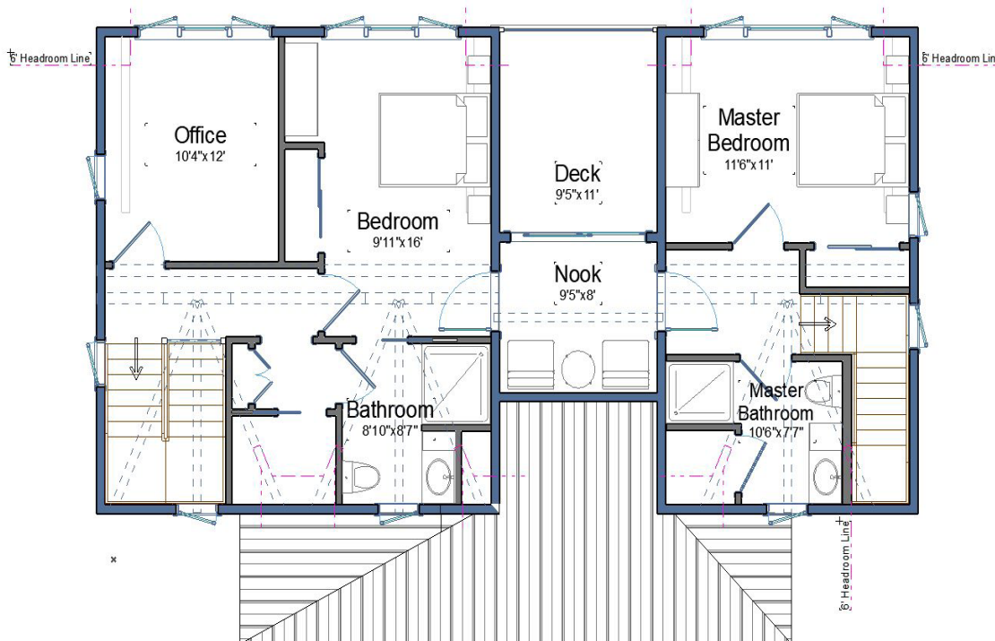
SECOND FLOOR
